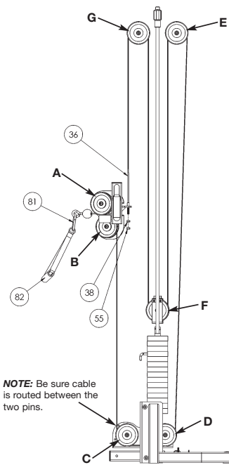
CABLE ROUTING DETAIL
